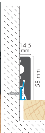
MOUNTING CLIP
