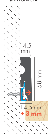
MOUNTING CLIP WITH SPACER
