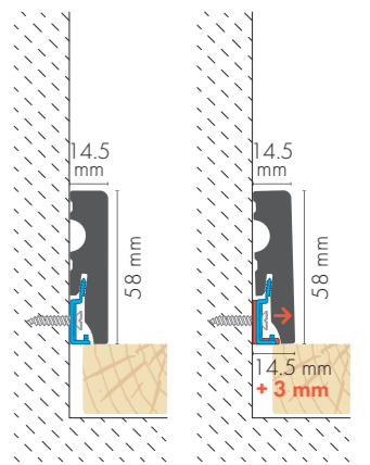
MOUNTING CLIP WITH SPACER
