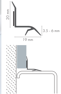
UO13 PVC Oval bathroom seal \frac{3}{4}
