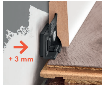
Assembly on a clip with spacer
