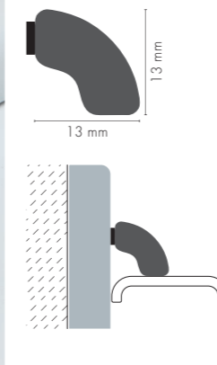
WNK PVC Edge profile
