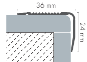
LSR24/ LSR24K ALU
