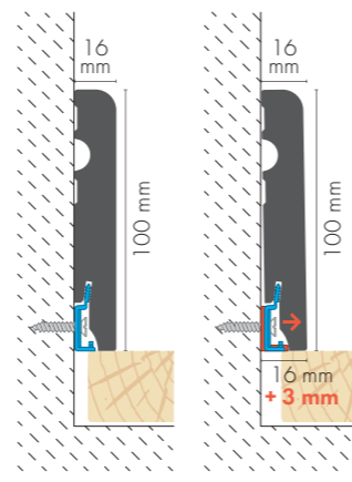
MOUNTING CLIP
