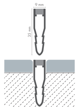
DY10G/ DY12G ALU Dilatation with black rubber
